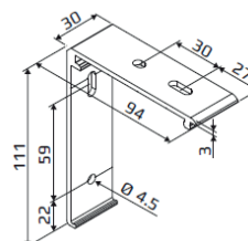
Monteringsclips
