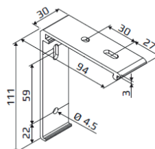
Monteringsclips
