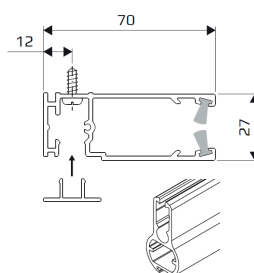
Monteringsclips
